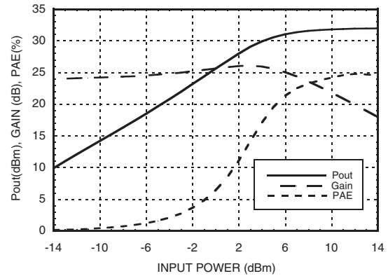
Power Compression @ 8 GHz, 7V @ 820 mA
