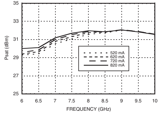
Psat vs. Current
