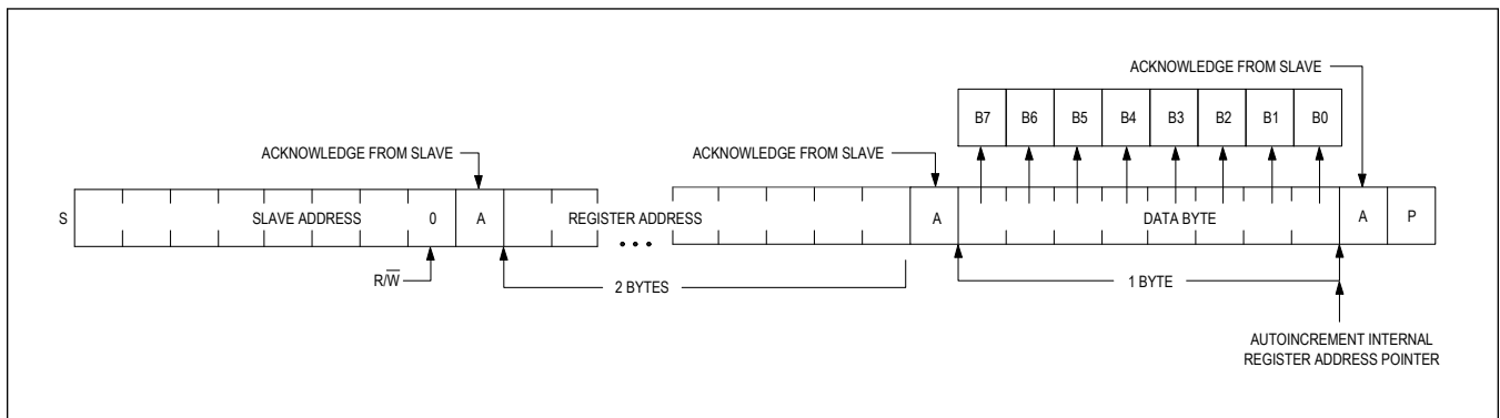
Figure 35. I 2 C Writing One Byte of Data to the Slave
