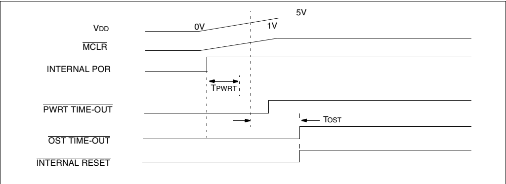
FIGURE 12-10: SLOW RISE TIME (MCLR TIED TO VDD)
