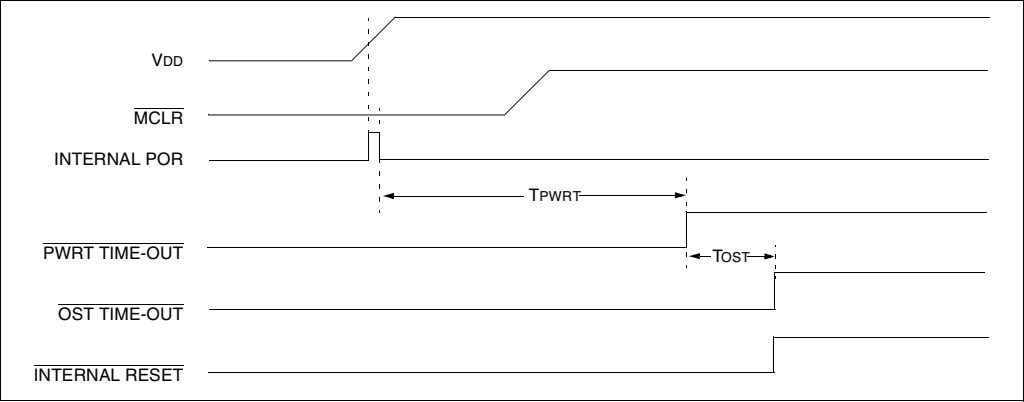
FIGURE 12-9: TIME-OUT SEQUENCE ON POWER-UP (MCLR NOT TIED TO VDD): CASE 2
