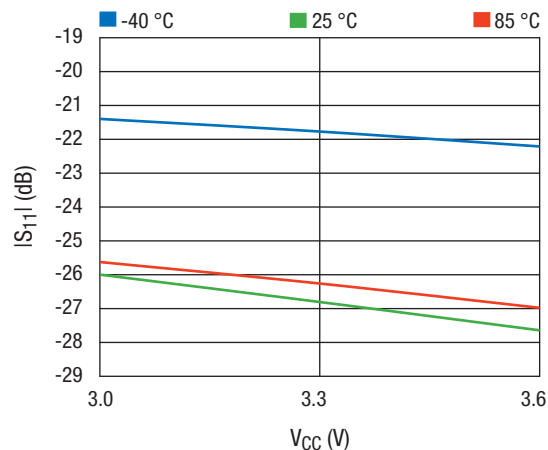
Figure 11. IS11I vs. VCC Across Temperature
