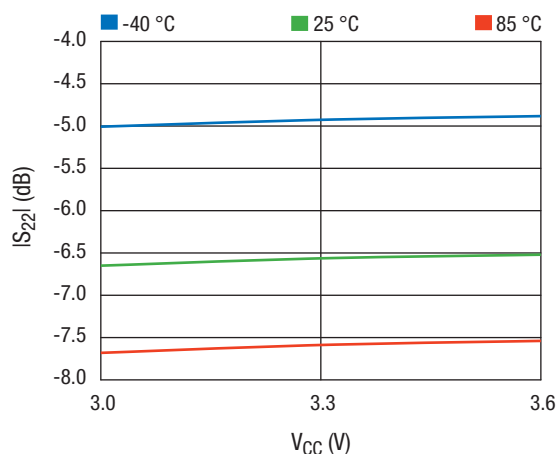
Figure 13. IS22I vs. VCC Across Temperature
