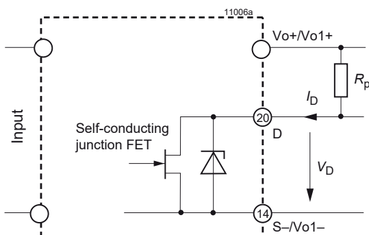
Fig. 35 Option D0 – D4: JFET output, I_D \leq 2.5 \text{ mA}
