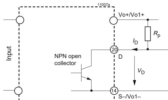
Fig. 36 Option D5 – DD: NPN output, V_D \leq 40, I_D \leq 2.5 mA
