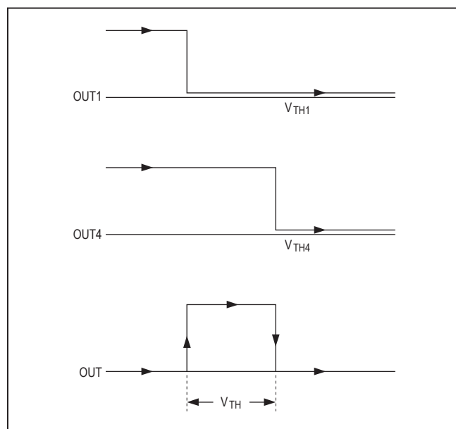
Figure 4. Output Response of Window Detector Circuit
