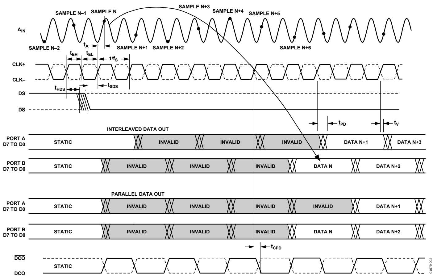
Figure 2. Timing Diagram
