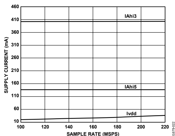
Figure 22. Power Supply Currents vs. Sample Rate
