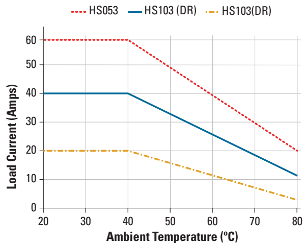
DP Series Derating Curve
