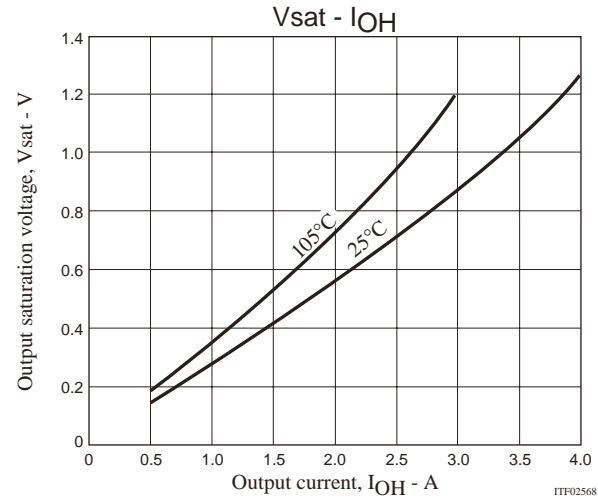
STK672-540 Forward voltage, V_{df} - Output current, I_{OH}
