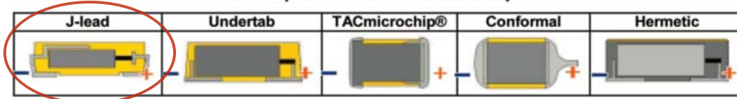
Five Capacitor Construction Styles
