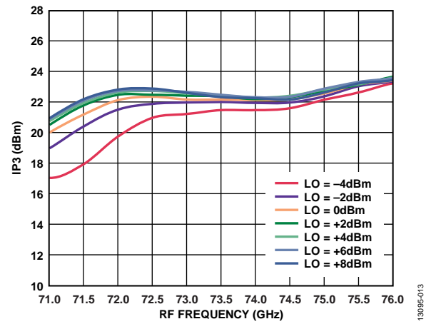
Figure 13. Input IP3 vs. RF Frequency at Various LO Powers, I_{FIN} = 5 dBm, IF = 1000 MHz, LSB
