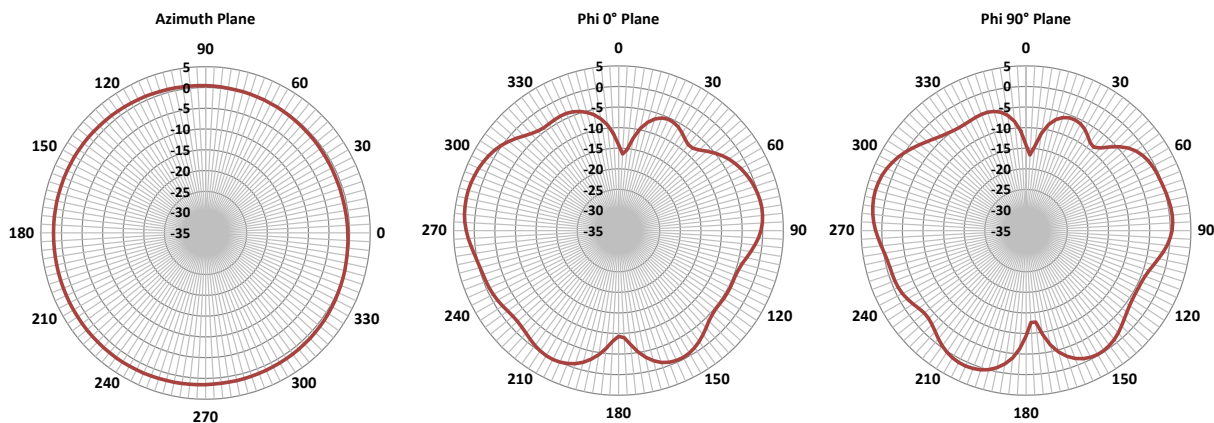
Radiation Pattern at 2110 MHz
