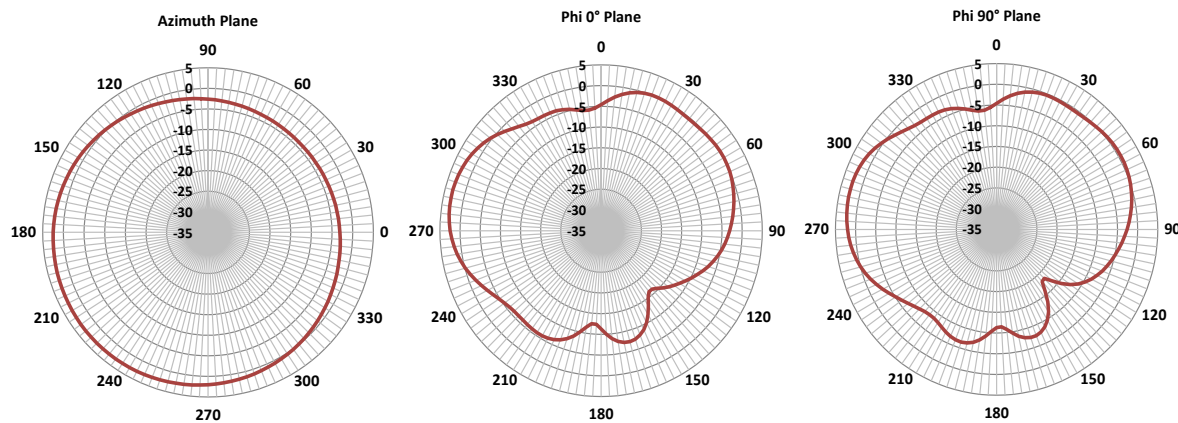
Radiation Pattern at 2700 MHz
