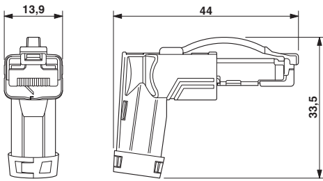
RJ45 plug-in connector, IP20, angled
