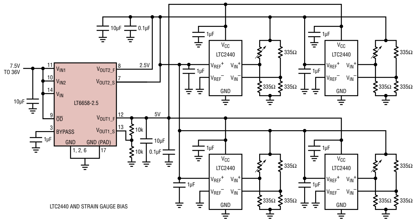
LT6658 Biasing Multiple Strain Gauges
