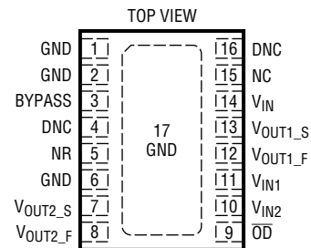
DE PACKAGE 16-LEAD (4mm x 3mm) PLASTIC DFN
