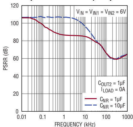
2.5V V_{OUT2} Power Supply Rejection Ratio vs Frequency
