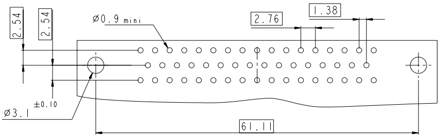
LAYOUT DIMENSIONS
