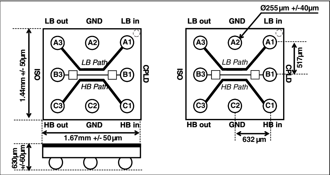
Figure 11. Package dimensions
