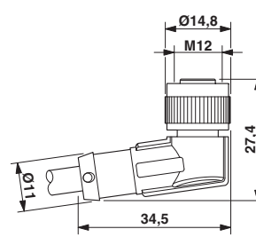
Dimensioned drawing
