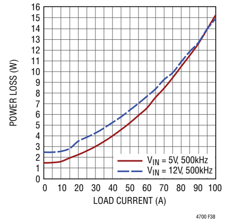
Figure 38. 1.8V Power Loss Curve
