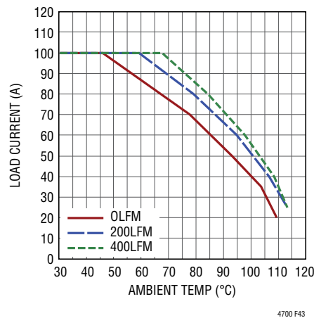
Figure 43. 5V to 1.8V Derating Curve, No Heat Sink
