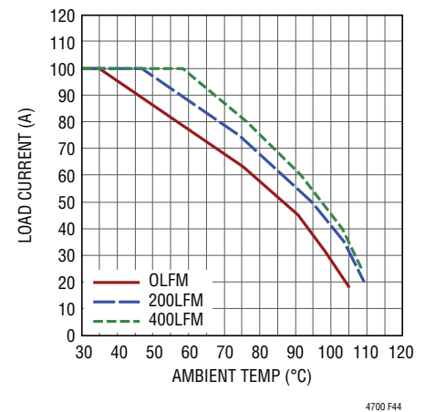
Figure 44. 12V to 1.8V Derating Curve, No Heat Sink
