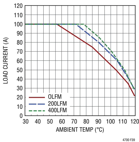
Figure 39. 5V to 0.8V Derating Curve, No Heat Sink
