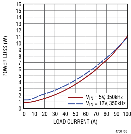
Figure 36. 0.8V Power Loss Curve
