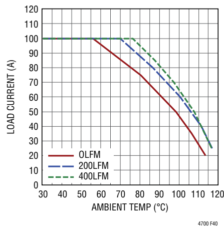
Figure 40. 12V to 0.8V Derating Curve, No Heat Sink
