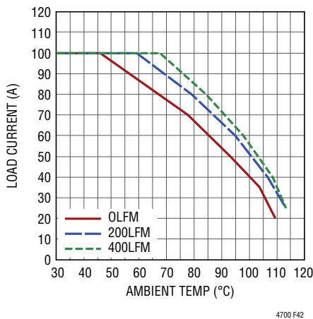
Figure 42. 12V to 1.2V Derating Curve, No Heat Sink
