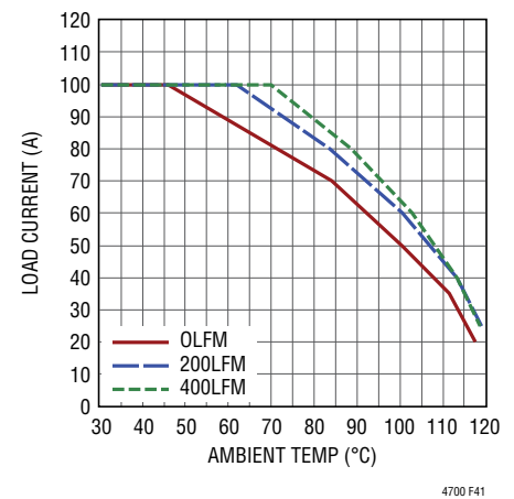
Figure 41. 5V to 1.2V Derating Curve, No Heat Sink
