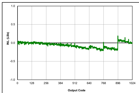
FIGURE 38-5: ADC 10-bit Mode, Single-Ended INL, V_{DD} = 3.0V , V_{REF} = 3.0V , T_A = 25^\circ\text{C} , T_{AD} = 4\text{ }\mu\text{S} .
