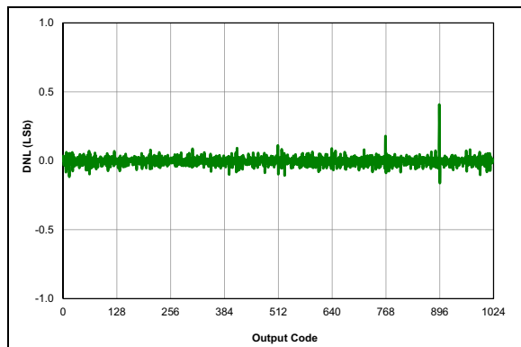
FIGURE 38-3: ADC 10-bit Mode, Single-Ended DNL, V_{DD} = 3.0V , V_{REF} = 3.0V , T_A = 25^\circ\text{C} , T_{AD} = 8\text{ }\mu\text{S} .
