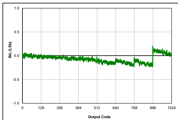
FIGURE 38-6: ADC 10-bit Mode, Single-Ended INL, V_{DD} = 3.0V , V_{REF} = 3.0V , T_A = 25^\circ\text{C} , T_{AD} = 8\text{ }\mu\text{S} .
