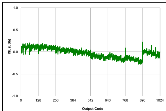
FIGURE 38-4: ADC 10-bit Mode, Single-Ended INL, V_{DD} = 3.0V , V_{REF} = 3.0V , T_A = 25^\circ\text{C} , T_{AD} = 1\text{ }\mu\text{S} .
