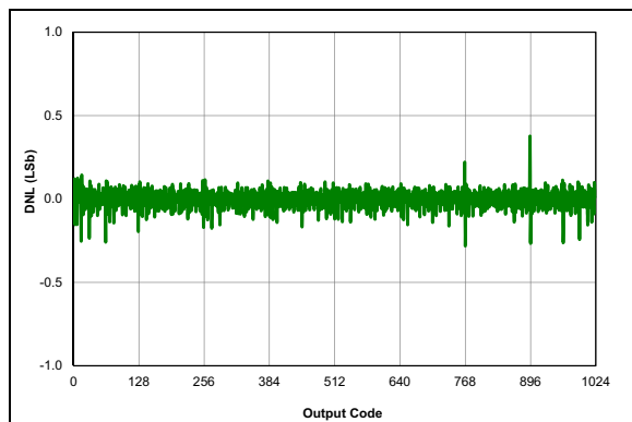
FIGURE 38-1: ADC 10-bit Mode, Single-Ended DNL, V_{DD} = 3.0V , V_{REF} = 3.0V , T_A = 25^\circ\text{C} , T_{AD} = 1\text{ }\mu\text{S} .
