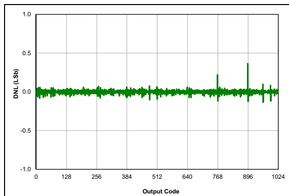
FIGURE 38-2: ADC 10-bit Mode, Single-Ended DNL, V_{DD} = 3.0V , V_{REF} = 3.0V , T_A = 25^\circ\text{C} , T_{AD} = 4\text{ }\mu\text{S} .
