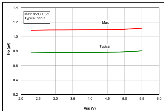
FIGURE 38-76: I_{PD} , Watchdog Timer (WDT), PIC16LF15354/55 devices only
