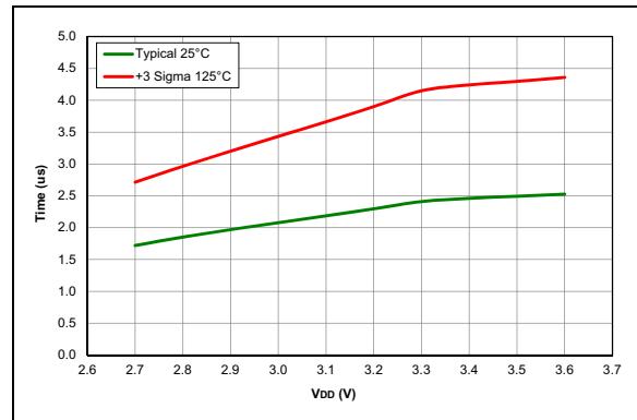
FIGURE 38-22: Brown-out Reset Response Time, PIC16LF15354/55 devices only.
