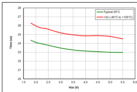
FIGURE 38-102: Wake from Sleep, V_{REGPM} = 1 , HFINTOSC = 16\text{ MHz} , PIC16F15354/55 devices only
