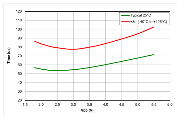
FIGURE 38-101: Wake from Sleep, V_{REGPM} = 1 , HFINTOSC = 4\text{ MHz} , PIC16F15354/55 devices only
