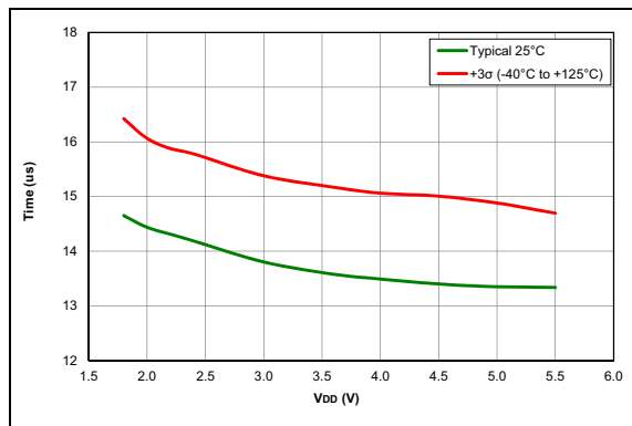
FIGURE 38-100: Wake From Sleep, V_{REGPM} = 0 , HFINTOSC = 4\text{ MHz} , PIC16F15354/55 devices only
