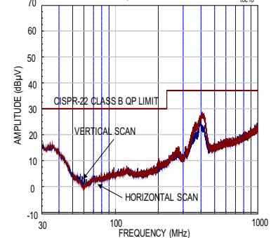
RADIATED EMI CURVE 5V OUTPUT, 3.5A LOAD CURRENT
