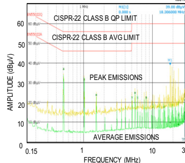
CONDUCTED EMI CURVE 5V OUTPUT, 3.5A LOAD CURRENT
