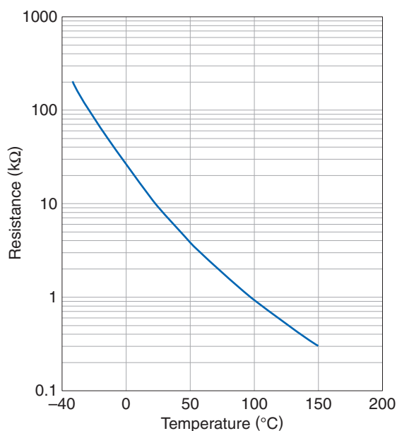
Fig.1 R-T Curve : 10k \Omega m@25°C
