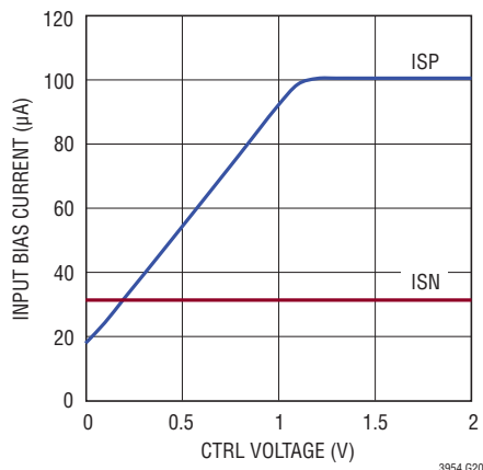
ISP/ISN Input Bias Current vs CTRL Voltage, I_{SP} = 24\text{V}
