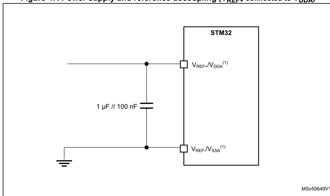
Figure 47. Power supply and reference decoupling ( V_{REF+} connected to V_{DDA} )
