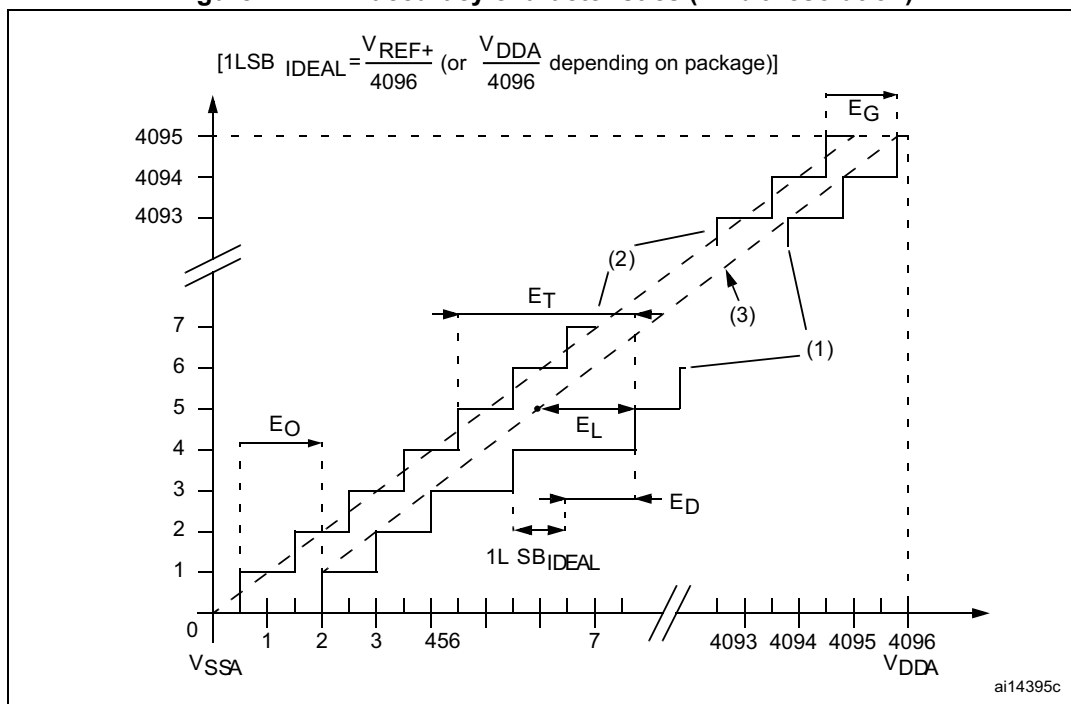
Figure 44. ADC accuracy characteristics (12-bit resolution)
