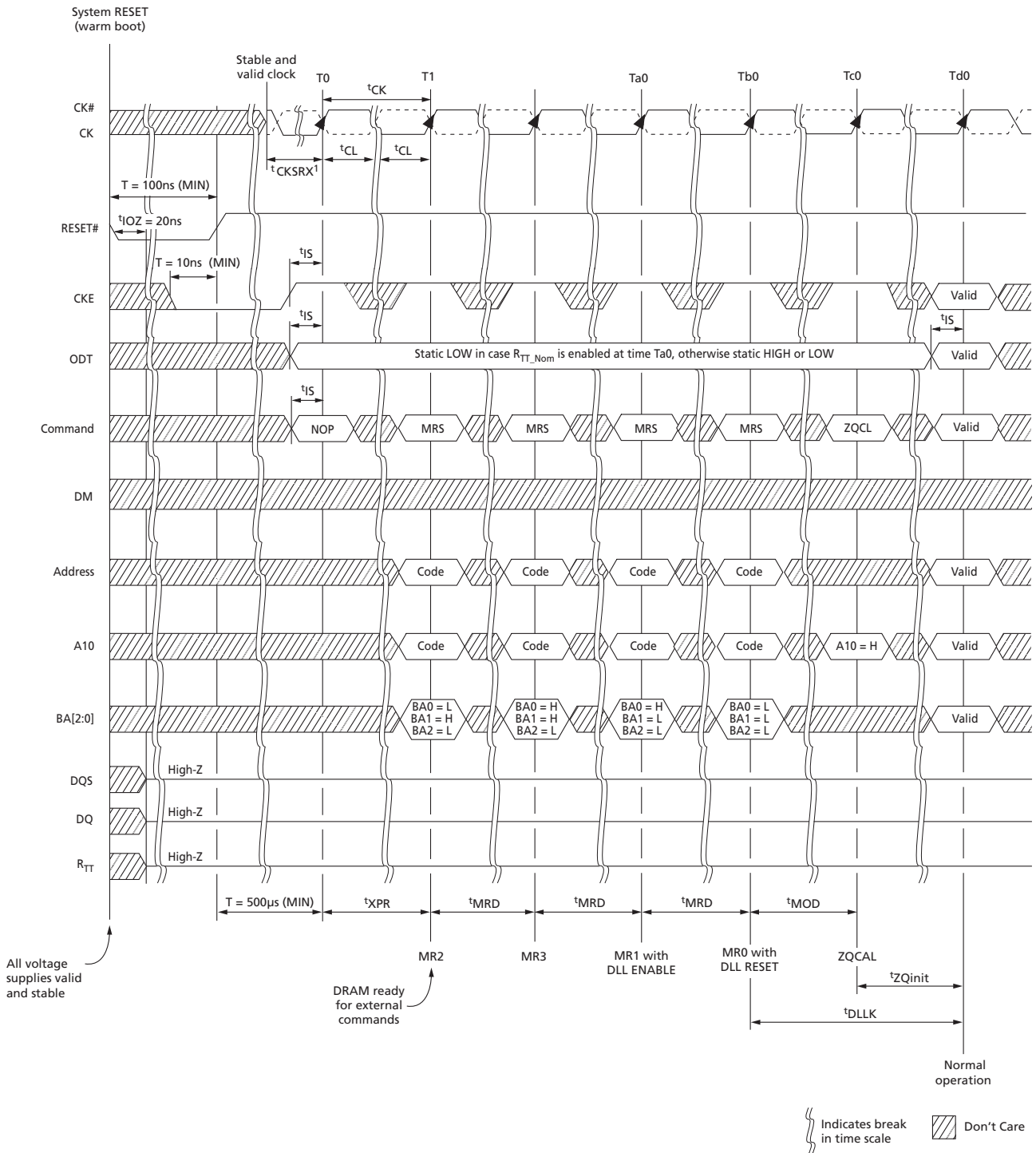
Figure 109: RESET Sequence
