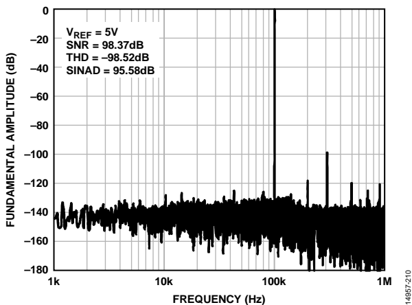
Figure 14. 100 kHz, -0.5 dBFS Input Tone FFT, Wide View
