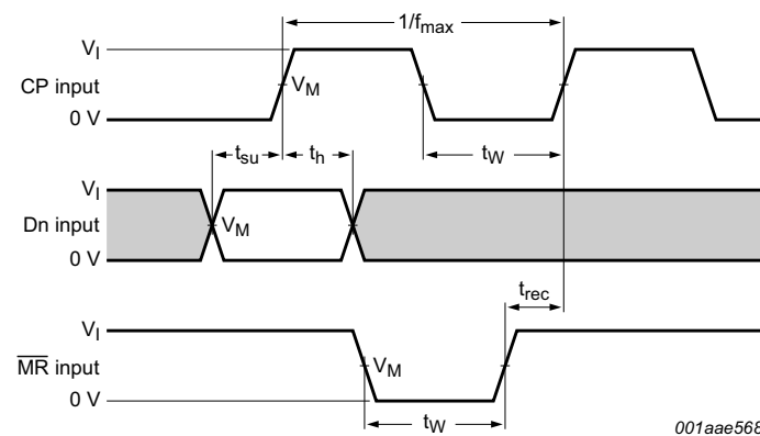
b. Minimum pulse widths for CP and \overline{\text{MR}} , \overline{\text{MR}} to CP recovery time, and set-up and hold time for Dn to CP
