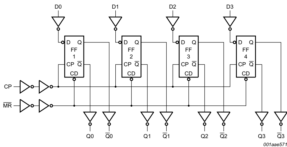
Fig 2. Logic diagram
