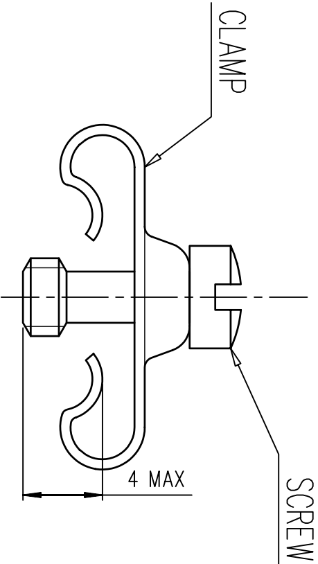
ASSEMBLY VIEW
