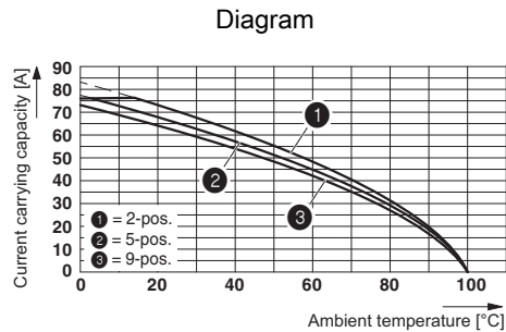
Type: ISPC 16/...-ST-10,16 with SPC 16/...-ST-10,16
