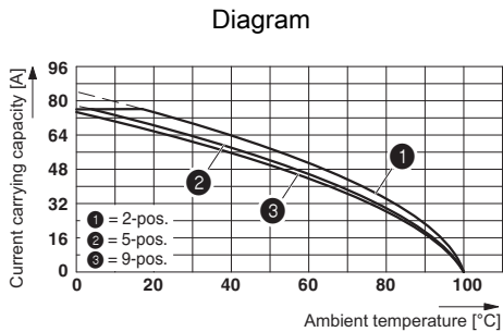
Type : ISPC 16/...-ST-10,16 with IPC 16/...-G-10,16
