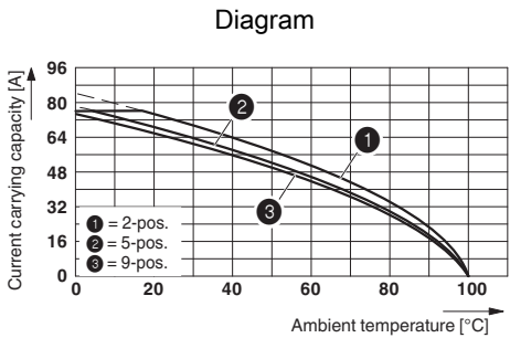
Derating curve for: ISPC 16/...-ST-10,16 with IPCV 16/...-G-10,16
