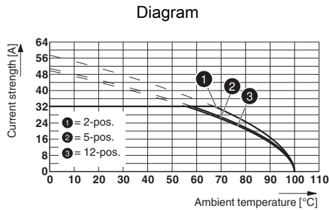
Type: ISPC 16/...-ST-10,16 with DFK-IPC 16/...-ST-10,16
