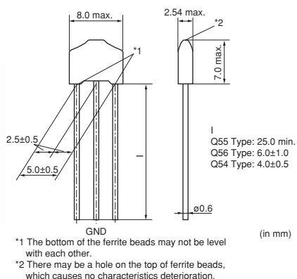
DSS6_Q55B Series Straight Type
