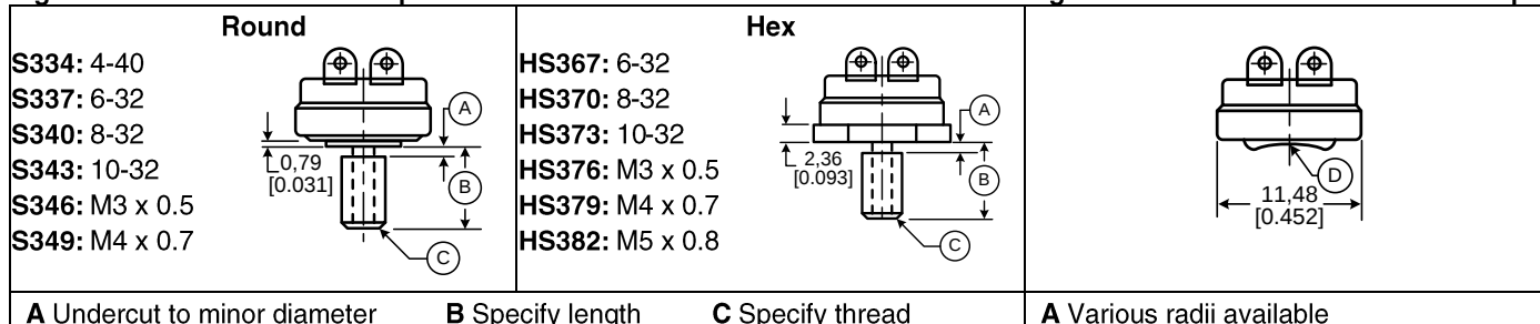
Figure 20. 3001/3004 Series Cap Studs
