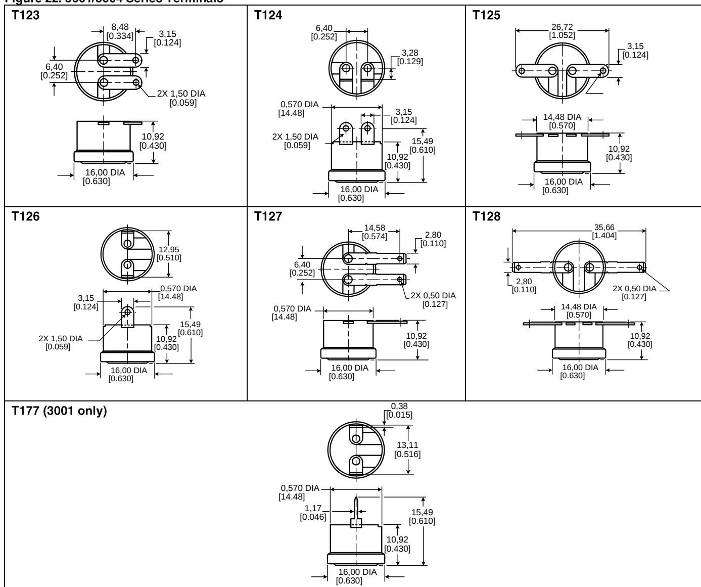
Figure 22. 3001/3004 Series Terminals
