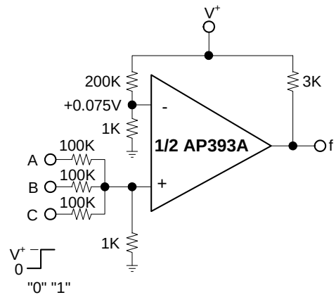
Or Gate
