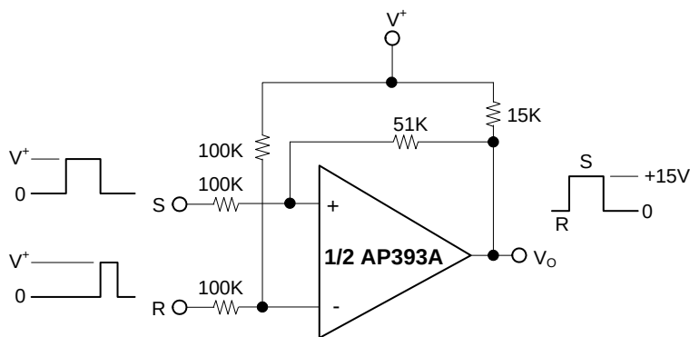
Bi-Stable Multivibrator
