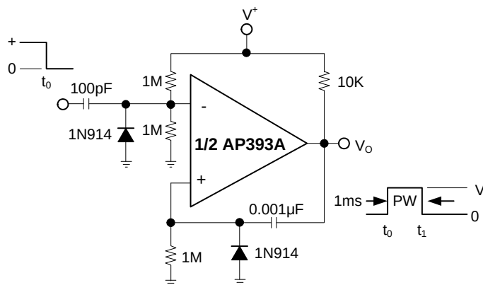
One-Shot Multivibrator
