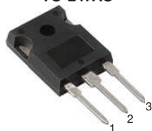
Base cathode 2 Anode 1 Anode 3 VS-40APS16PbF VS-40APS16-M3
