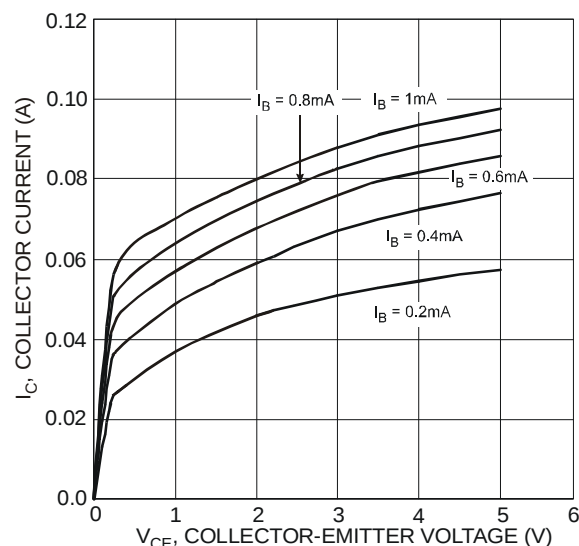
Fig. 4 Typical Collector Current vs. Collector-Emmitter Voltage
