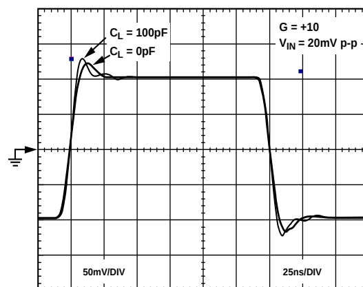
Figure 19. Small Signal Transient Response \pm 5\text{V} Supply
