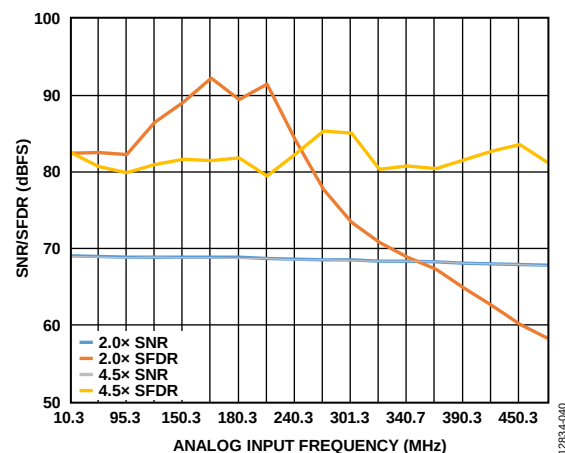
Figure 40. SNR/SFDR vs. f_{IN} ; f_{IN} < 500 MHz; Buffer Control 1 (0x018) = 2.0\times and 4.5\times
