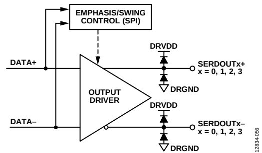
Figure 56. Digital Outputs
