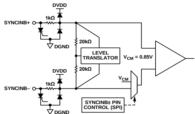
Figure 57. SYNCINB± Inputs
