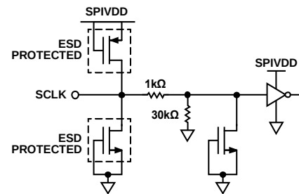
Figure 58. SCLK Input
