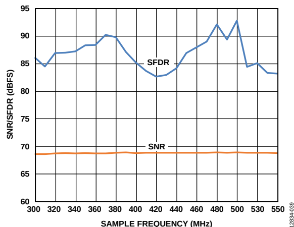
Figure 39. SNR/SFDR vs. f_s , f_{IN} = 170.3 MHz; Buffer Control 1 = 2.0\times
