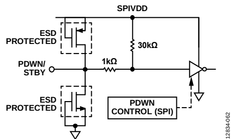
Figure 62. PDWN/STBY Input
