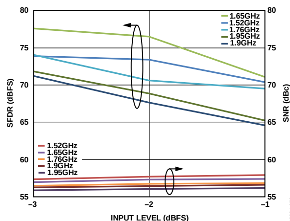
Figure 70. SNR/SFDR vs. Analog Input Level vs. Input Frequencies, AD9690-1000
