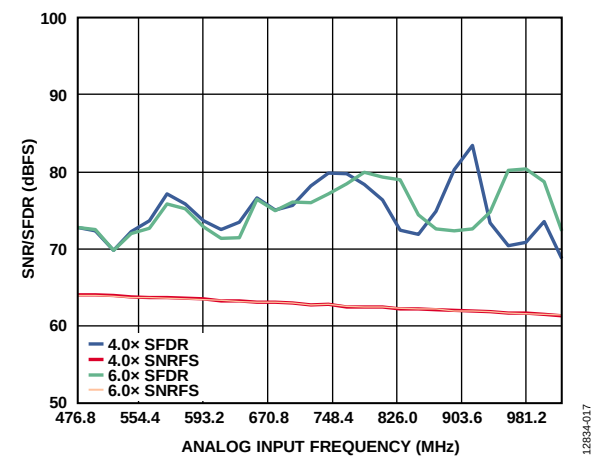
Figure 17. SNR/SFDR vs. Analog Input Frequency ( f_{IN} ); 500 \text{ MHz} < f_{IN} < 1 \text{ GHz} ; Buffer Control1 (0x018) = 4.0x and 6.0x
