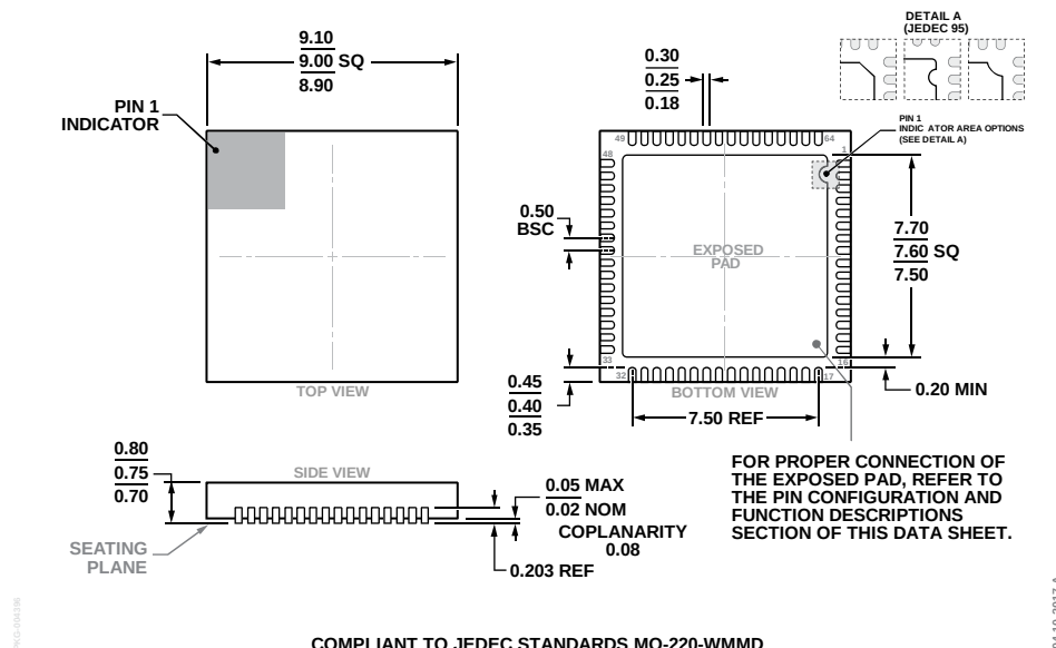
Figure 116. 64-Lead Lead Frame Chip Scale Package [LFCSP] 9 mm × 9 mm Body and 0.75 mm Package Height (CP-64-15) Dimensions shown in millimeters
