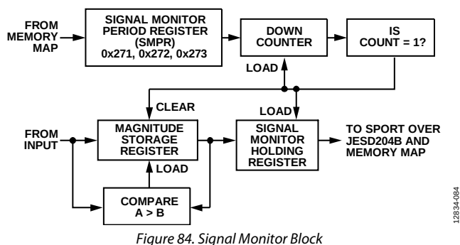
Figure 84. Signal Monitor Block
