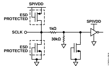
Figure 58. SCLK Input
