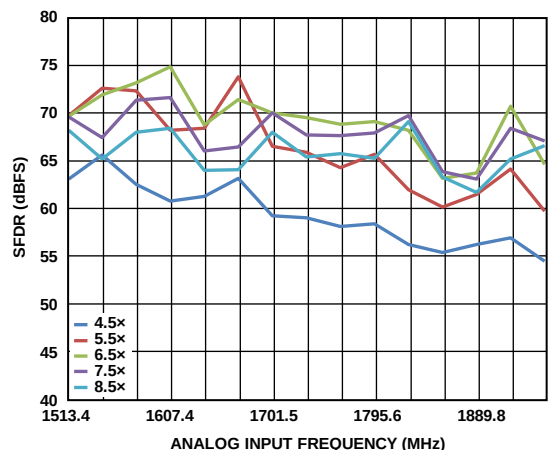
Figure 69. Buffer Current Sweeps, AD9690-1000 (SFDR vs. I_{BUFF} ); 1500 \text{ MHz} < f_{IN} < 2000 MHz; Front-End Network Shown in Figure 64
