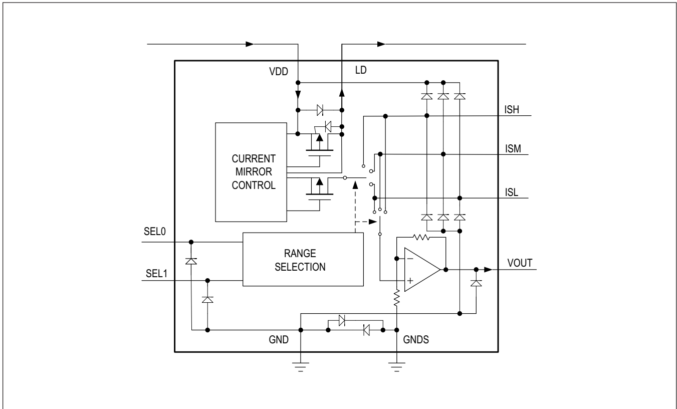
Figure 1. Functional Diagram Showing ESD Clamps
