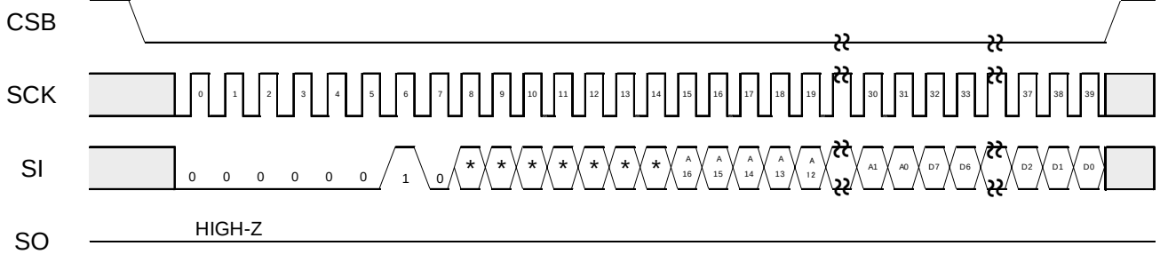
Figure 34. Write command
