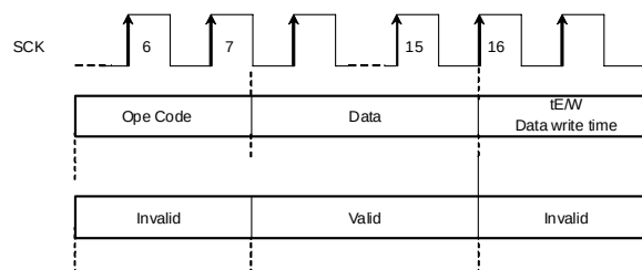
Figure 37. WPB valid timing (At inputting WRSR command)
