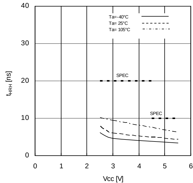
Figure 25. HOLDB Release Hold Time vs Supply Voltage
