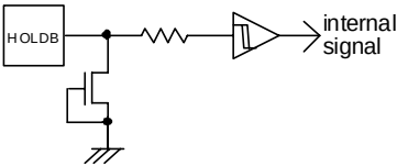
Figure 50. HOLDB input equivalent circuit
