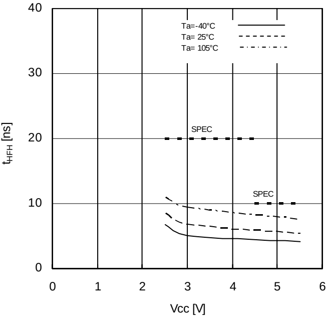
Figure 24. HOLDB Setting Hold Time vs Supply Voltage
