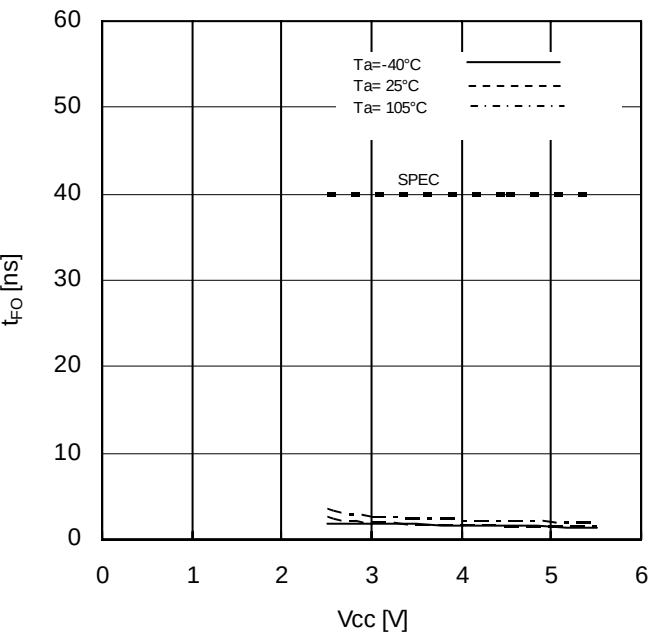
Figure 29. OUTPUT Fall Time vs Supply Voltage
