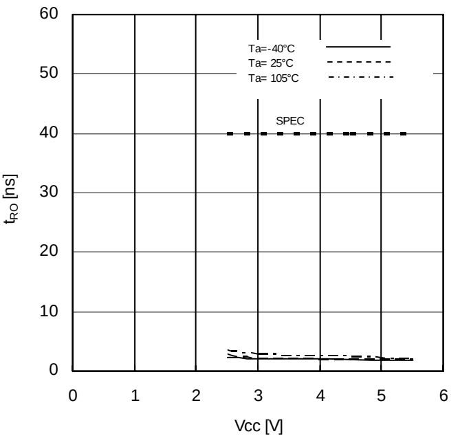
Figure 28. OUTPUT Rise Time vs Supply Voltage
