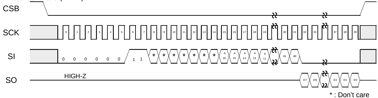
Figure 33. Read command
