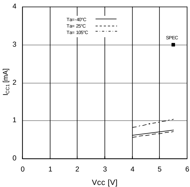
Figure 11. Supply Current (Write) vs Supply Voltage (fSCK=10MHz)
