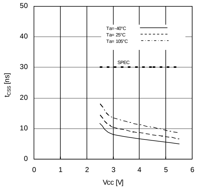
Figure 18. CSB Setup Time vs Supply Voltage
