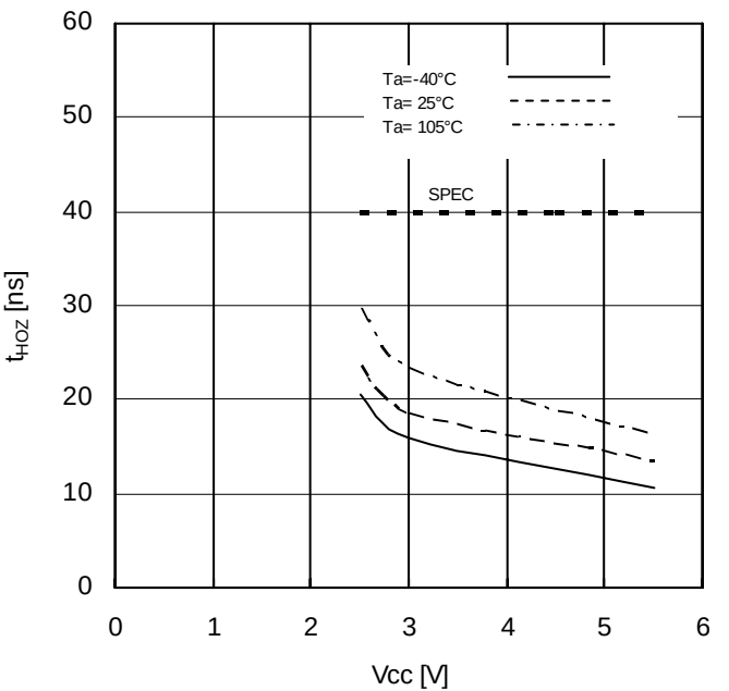
Figure 26. Time from HOLDB to Output High-Z vs Supply Voltage
