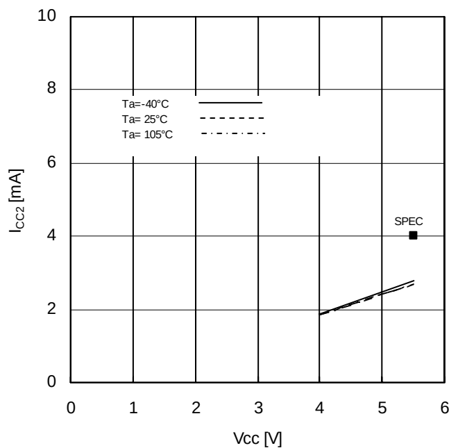
Figure 12. Supply Current (Read) vs Supply Voltage (fSCK=10MHz)
