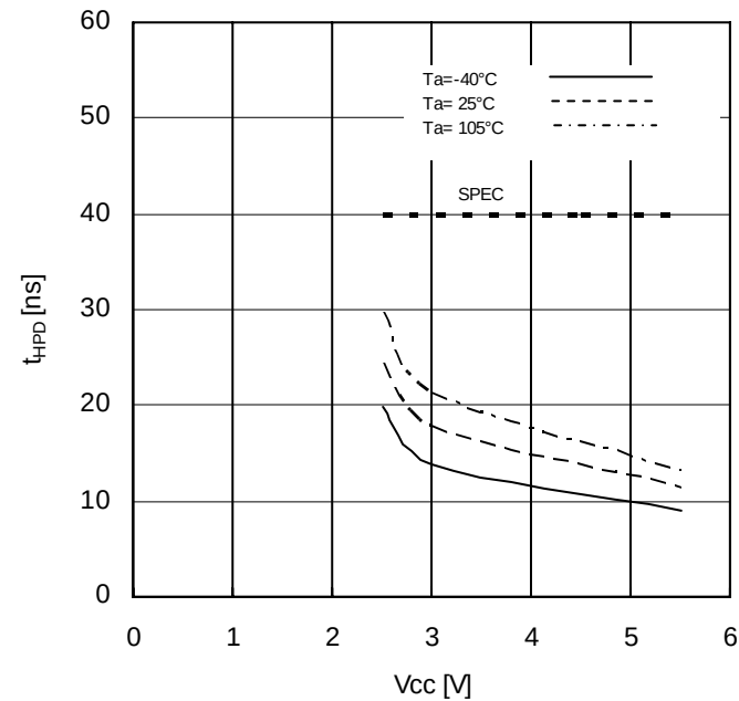
Figure 27. Time from HOLDB to Output change vs Supply Voltage
