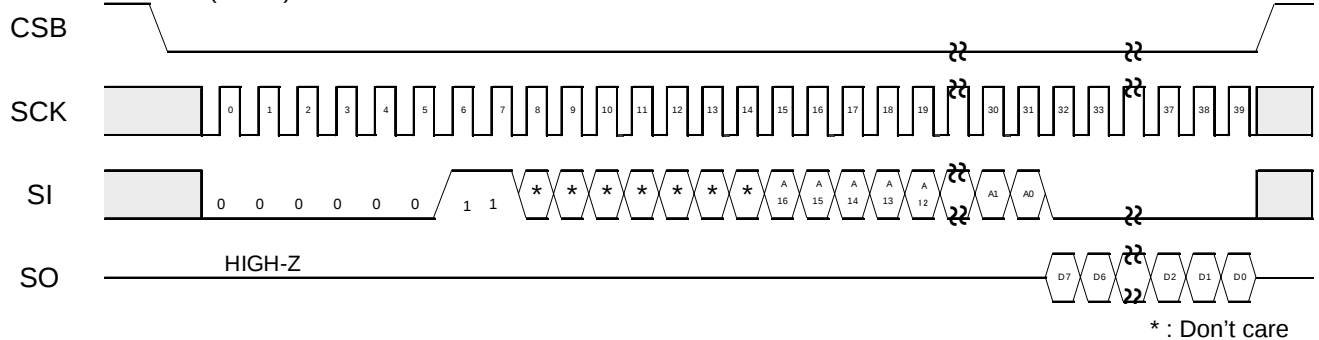
Figure 33. Read command
