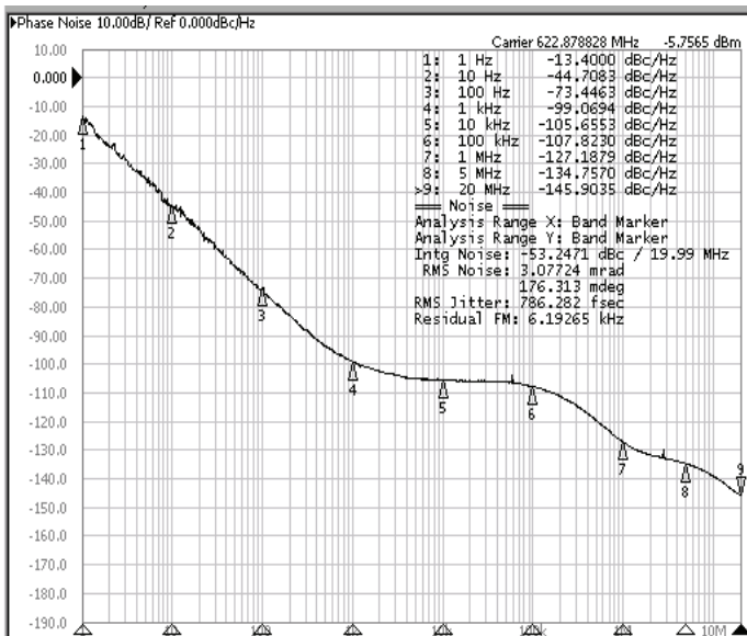
622.88MHz Carrier
