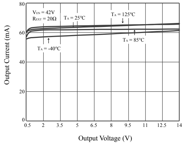
Figure 3 I_{OUT} vs. V_{OUT}
