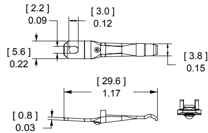
Ultra Short Contact
