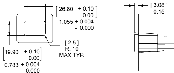
Panel Cut Out for All Receptacle Types
