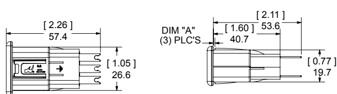
Flush Mount - For Solder Termination to Wire
