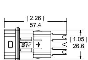
Short Depth - For Solder Termination to Wire
