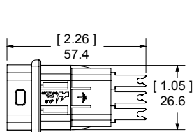
Short Depth - For Solder Termination to Wire
