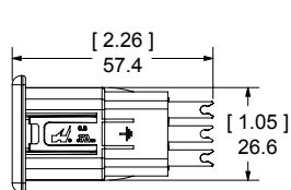
Flush Mount - For Solder Termination to Wire
