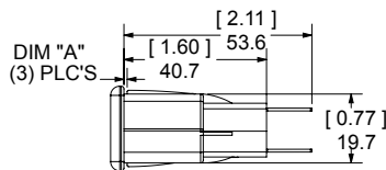
Flush Mount - For Solder Termination to Wire
