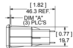
Flush Mount - For Solder Termination to PCB
