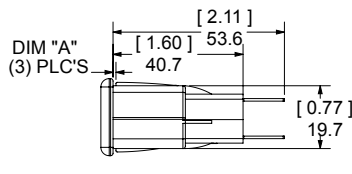
Flush Mount - For Solder Termination to Wire
