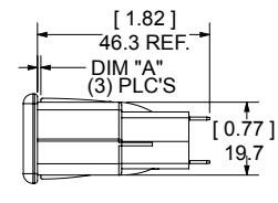
Flush Mount - For Solder Termination to PCB
