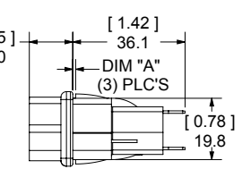
Short Depth - For Solder Termination to PCB
